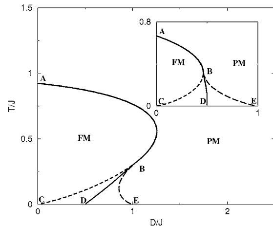
FIG. 3. Phase diagram (first-order transition and the spinodal lines) for the ordered BC model in the D - T plane for r=1 (inset, no inverse melting) and for r=6 (admits inverse melting, main figure). The value of r=6 has been chosen in order for the effect to be more pronounced, but inverse melting is seen as soon as r > 1 . AB is the second-order transition line, where B is the tricritical point. The line BD is the first-order transition line (the global minimum of the free energy is shifted from one phase to the other) while the lines BE and BC are the spinodal lines, where the local minima associated with one of the phases disappears.
