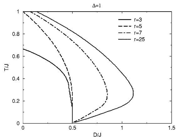
FIG. 12. Phase diagram for the mean-field version of the ordered model in the D - T plane. Here there is no exact degeneracy of the “interacting” states. Instead, r spin states are equally distributed around the \pm 1 state, with level spacing \Delta/r , as explained in the text. The first-order transition lines are plotted for different r 's, i.e., for different “density” of spin states inside a window of size \Delta . As seen in the figure, larger density of spin states corresponds to more pronounced inverse melting.
