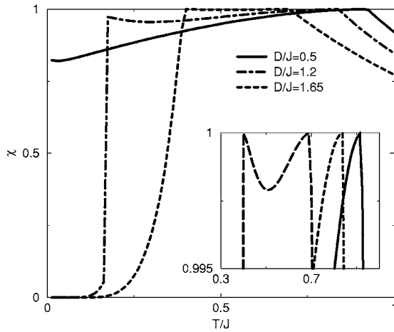
FIG. 9. Susceptibility as a function of the scaled temperature T/J for the glassy model for different values of D/J . First-order inverse melting shows an abrupt jump in the susceptibility while cusps are seen for all of the spin glass second-order transitions (as seen more clearly in the inset).
