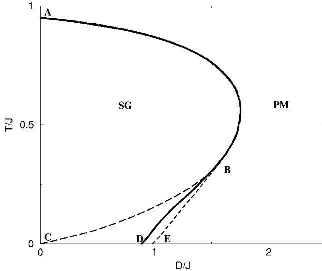
FIG. 8. Phase diagram, transition, and spinodal lines for the disordered model [see Eq. (13)] in the D-T plane for constant interaction J and degeneracy r=6 . The line ABD is a (normal and inverted) glass-transition line. To its left the spin glass phase admits a global minimum of the free energy (technically q \neq 0 ), while to its right the paramagnetic phase corresponds to that minimum ( q=0 ). AB is a second-order transition line and BD is a first-order transition line. BE and BC are the spinodal of the spin glass and of the paramagnetic phase, respectively.
