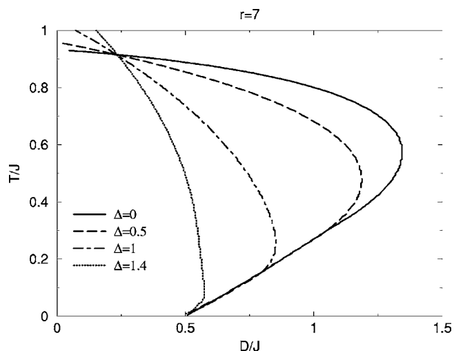
FIG. 13. The same as Fig. 12, but with a constant number of spin levels ( r = 7 ) for different widths \Delta around S = 1 . Again, a larger density of spin (hence energy) states implies inverse melting. The occurrence of two common points for all curves is discussed in the text.
