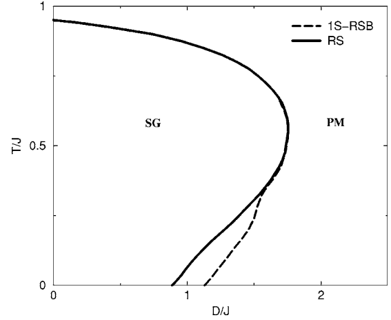
FIG. 11. First-order transition lines, separating regions of global stability for the glassy/paramagnetic phase, as obtained from the one-step RSB (dashed line) compared with the symmetric replica results (full line). The first-order transition is shifted to the right, but there is still a region of inverse glass transition.
