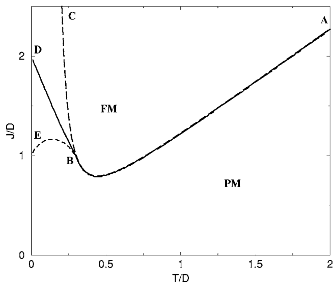
FIG. 4. First-order transition line (DBA) and spinodal lines (BC and BE) for the ordered BC model Eq. (3) in the T - J plane for r=6 . First- (BD) and second- (BA) order inverse melting of the first type are observed and the slope of the curve is negative.
